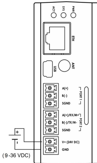
Figure 4 Power Connection Diagram
