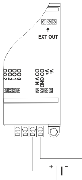
Figure 7 Power Connection Diagram
