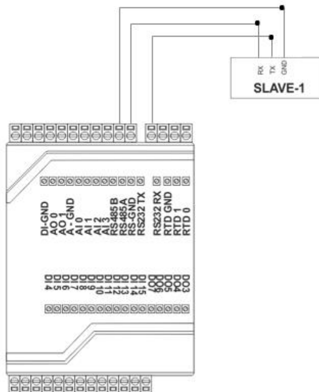
Figure 15 RS232 Serial Port Connection Diagram
