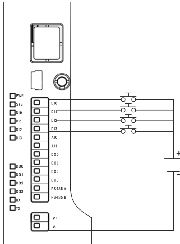
Figure 5 Digital Input Connection Diagram
