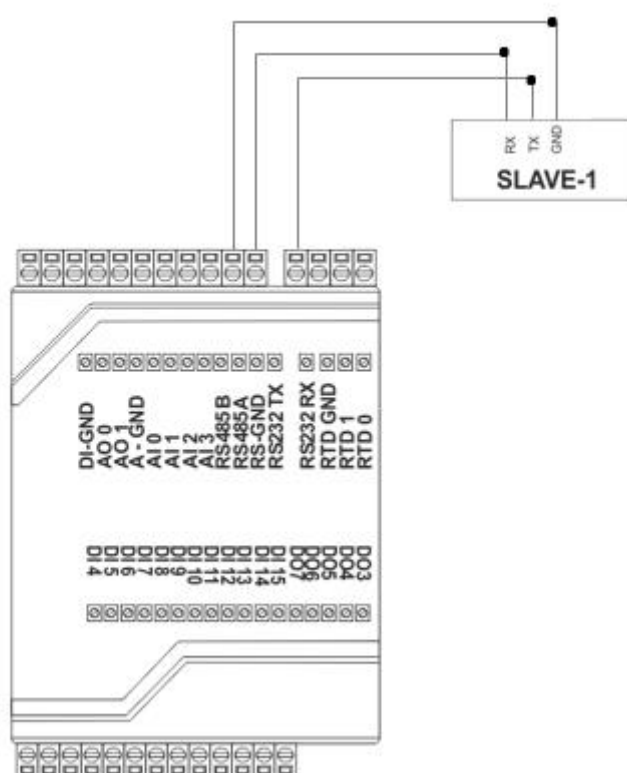
Figure 16 RTU300 RS232 Serial Port Connection Diagram
