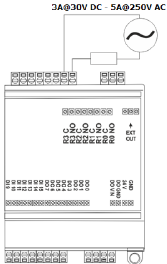
Figure 12 RTU300 Relay Connection Diagram
