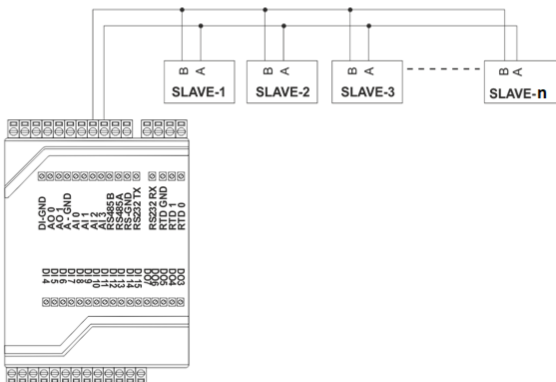
Figure 15 RTU300 RS485 Serial Port Connection Diagram
