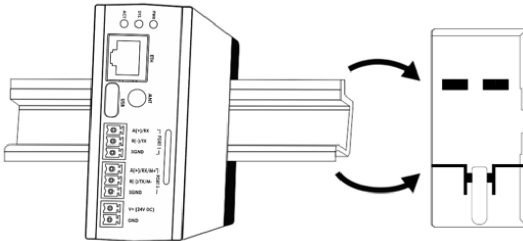
Figure 2 Mounting Information
