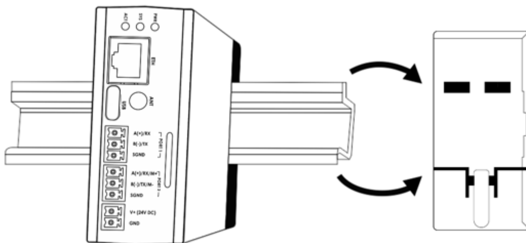
Figure 2 Mounting Information
