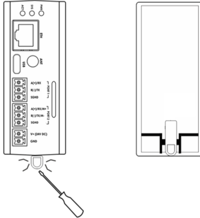
Figure 3 Demountage
