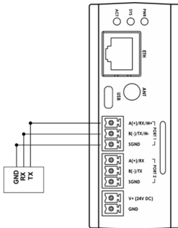
Figure 6 RS232 Input Connection Diagram
