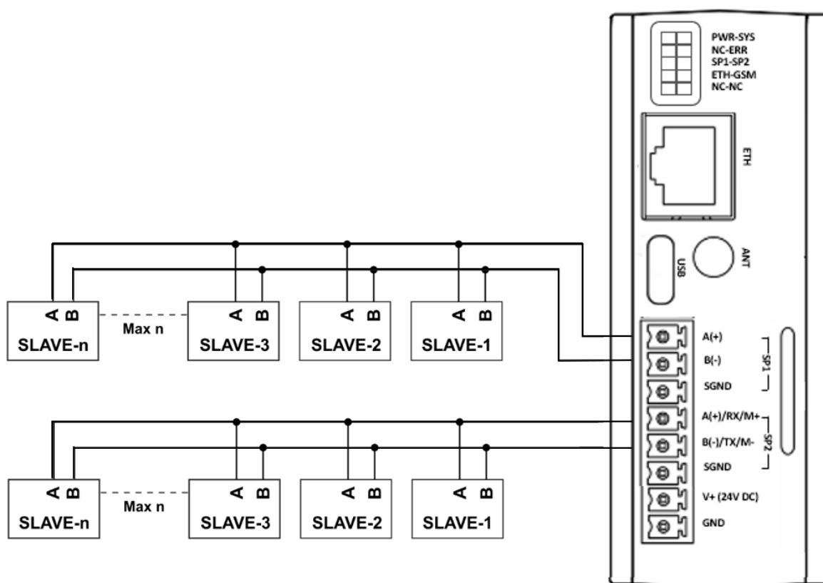
Figure 5 RS485 Input Connection Diagram
