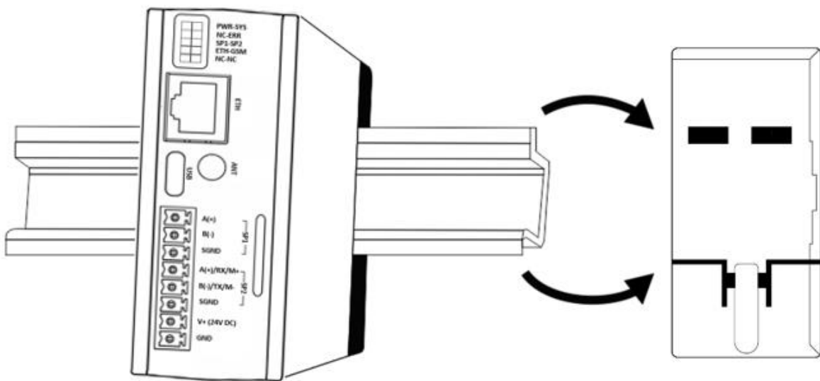
Figure 2 Mounting Information
