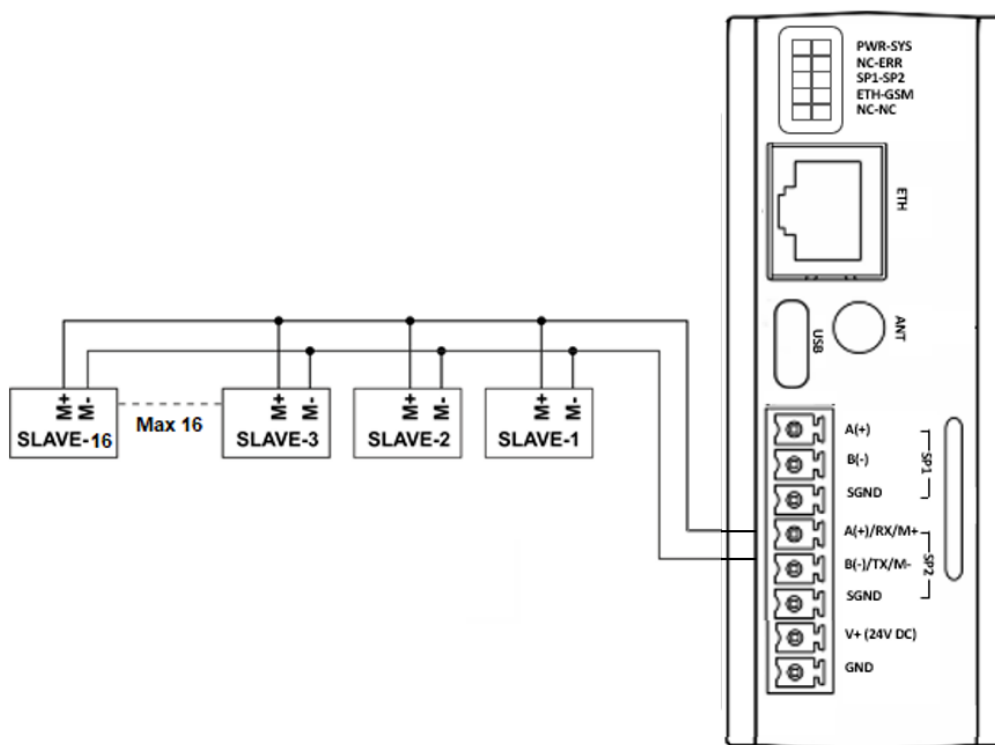
Figure 6 M-BUS Port Input Connection Diagram
