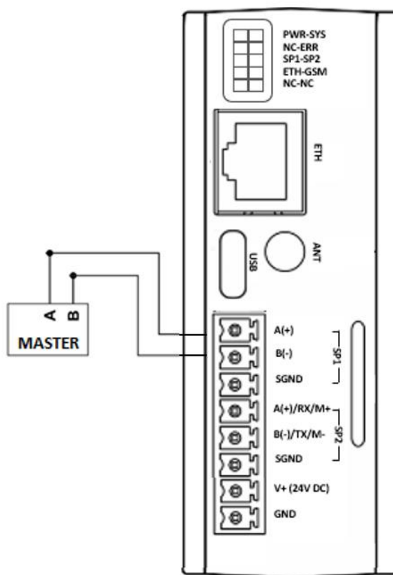
Figure 5 RS485 Port Input Connection Diagram
