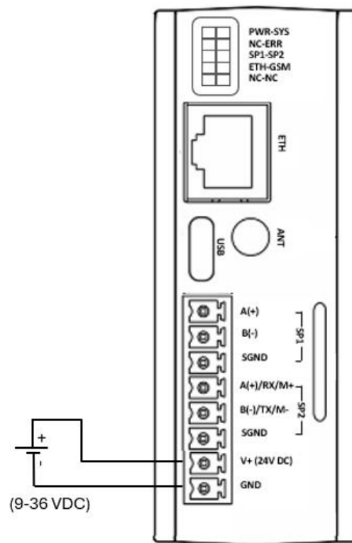
Figure 4 Power Connection Diagram
