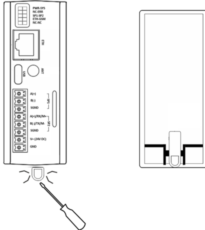
Figure 3 Demountage
