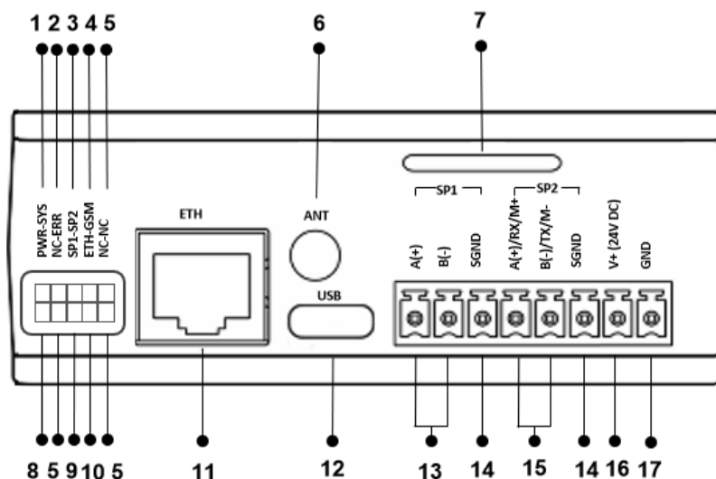
Figure 1 GC2 Board Type Connector and Physical Interfaces
