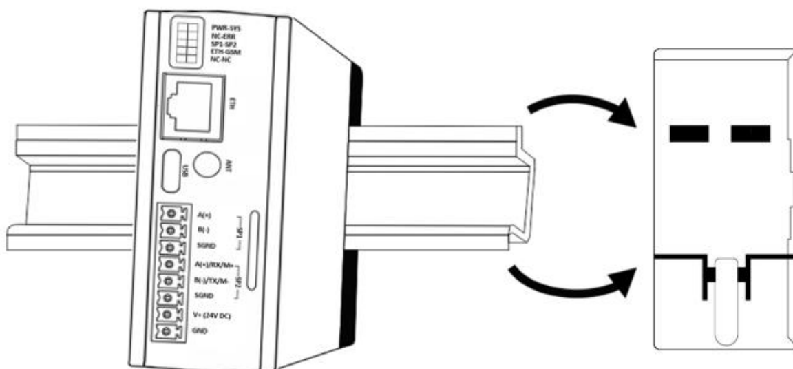
Figure 2 Mounting Information
