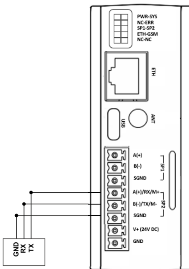
Figure 6 RS232 Input Connection Diagram
