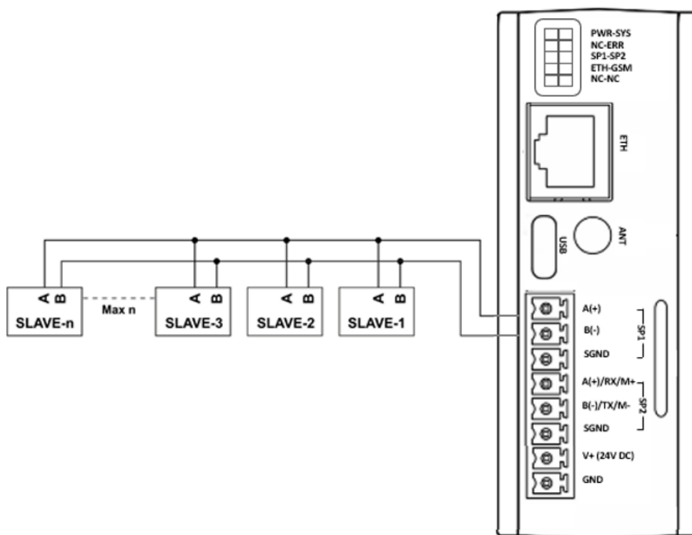
Figure 5 RS485 Input Connection Diagram
