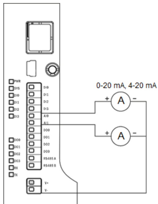
Figure 8 Analog Input Connection Diagram
