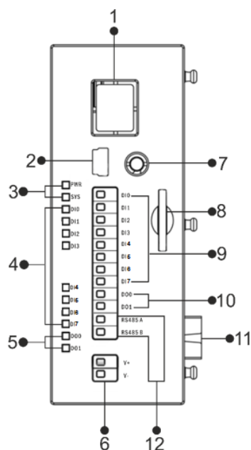
Figure 2 GB1 Board Type Connector and Physical Interface
